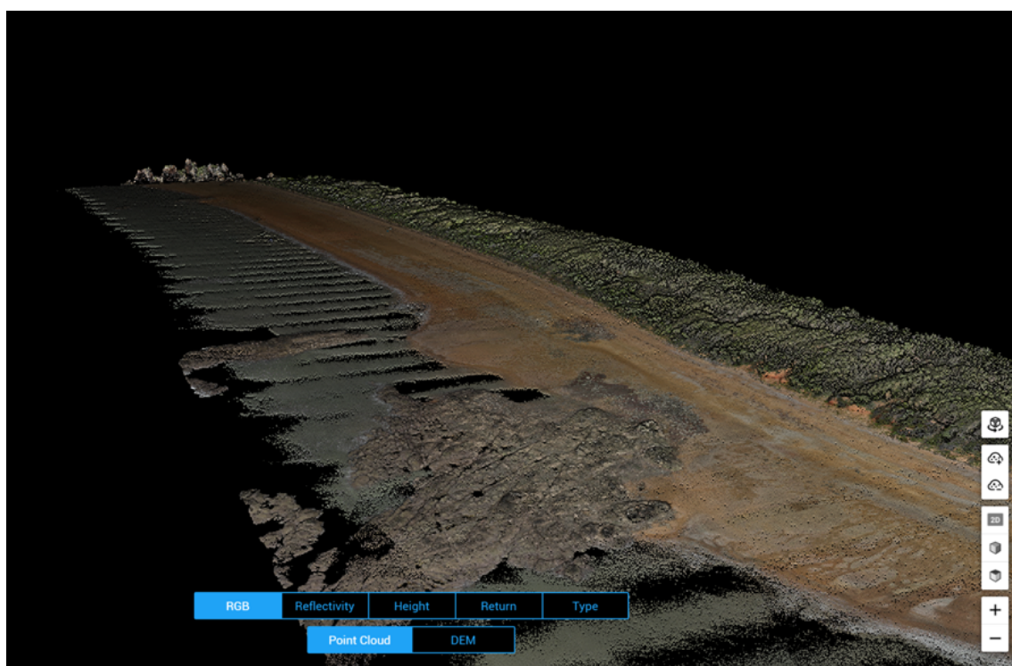
FIGURE 21: Aerial drone LiDAR Point Cloud output for Cape Domett Seaward Beach at spring low tide. These were used to create high resolution Digital Surface Model (DSM) and Digital Elevation Model (DEM) plus high-resolution photogrammetry of the four high-priority beaches. This provides a powerful baseline for long-term monitoring of these areas. The data and outputs are available to DBCA.
