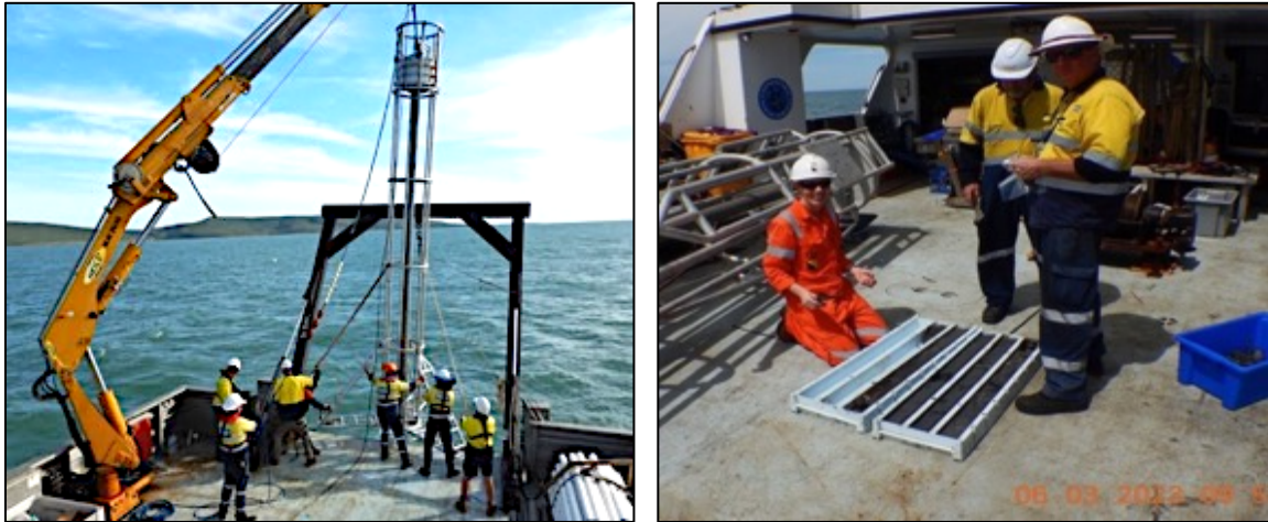
FIGURE 5.8: Vibro-core sampling in Block 4 during the Sand Exploration Survey in March 2023 (images: Raaymakers).
