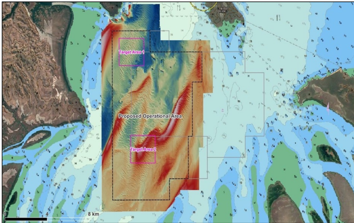
FIGURE 5.10: High resolution Multi-beam Echo Sounder (MBES) survey of the POA and 1 km buffer showing the seabed sand-forms in this area. Red indicates higher (shallower) bathymetry and thicker (deeper) bodies of sand.
