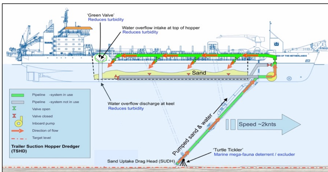
FIGURE 1.1: The proposed sand sourcing operation will involve a single Sand Production Vessel (SPV) based generally on the design of a large Trailer Suction Hopper Dredger (TSHD) shown here – but designed and built specifically for this project.
