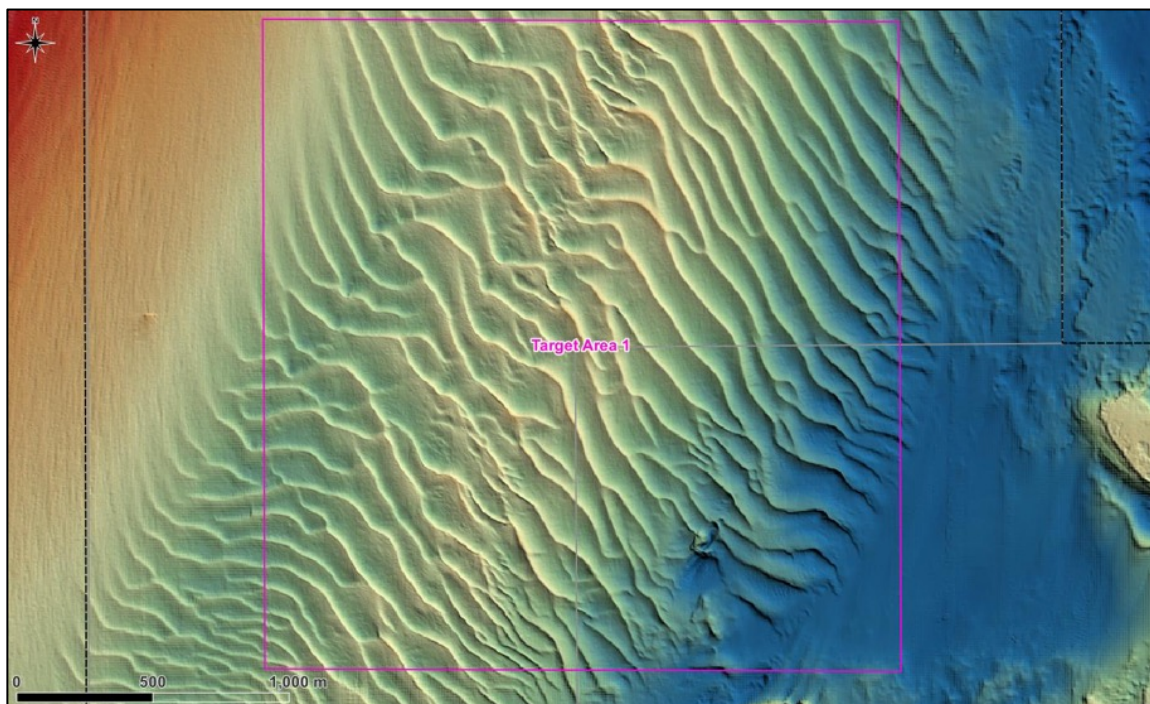
FIGURE 5.11: Digital elevation model generated from the high-resolution MBES of Target Area 1 in the POA showing the seabed sand waves. The sand waves have vertical heights ranging from 1 to 8 m and horizontal wavelengths of between 50 and 200 m.
