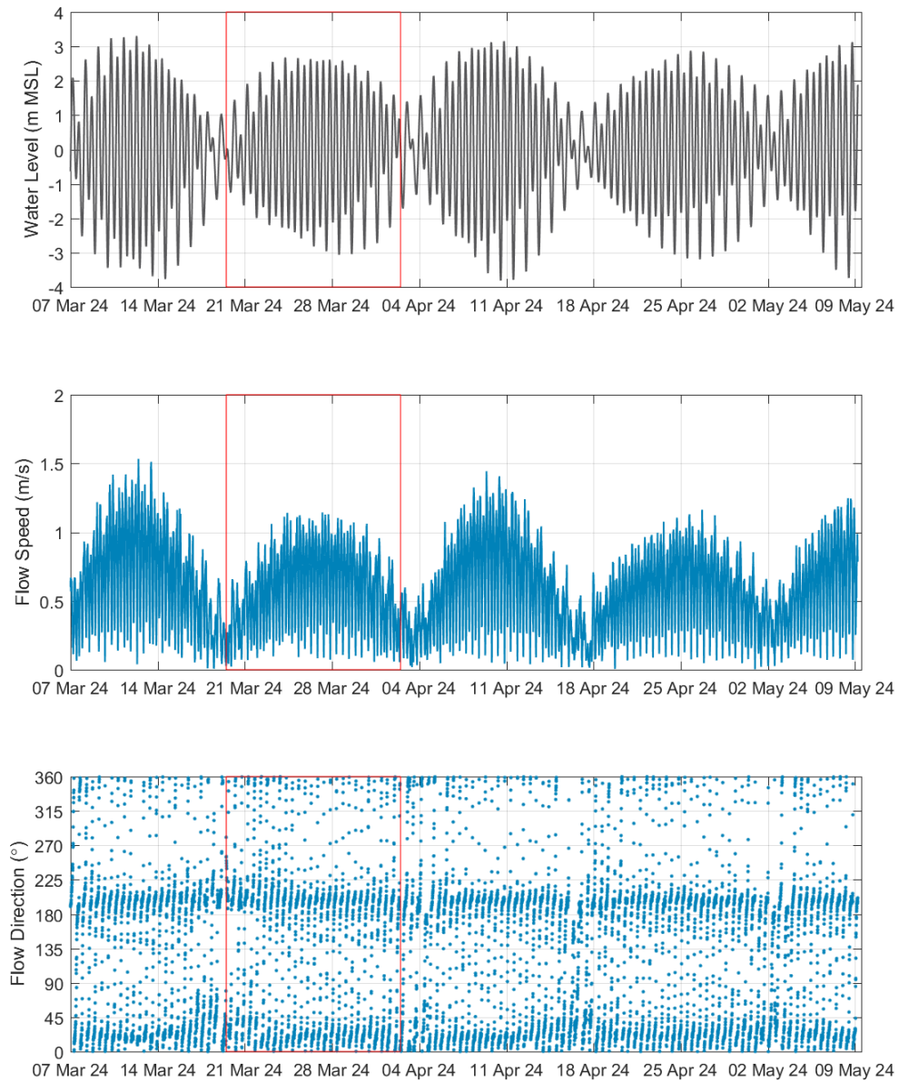
Figure 23. Hydrodynamic survey results for site AWAC-06, 6 th Mar to 10 th May 2024.
