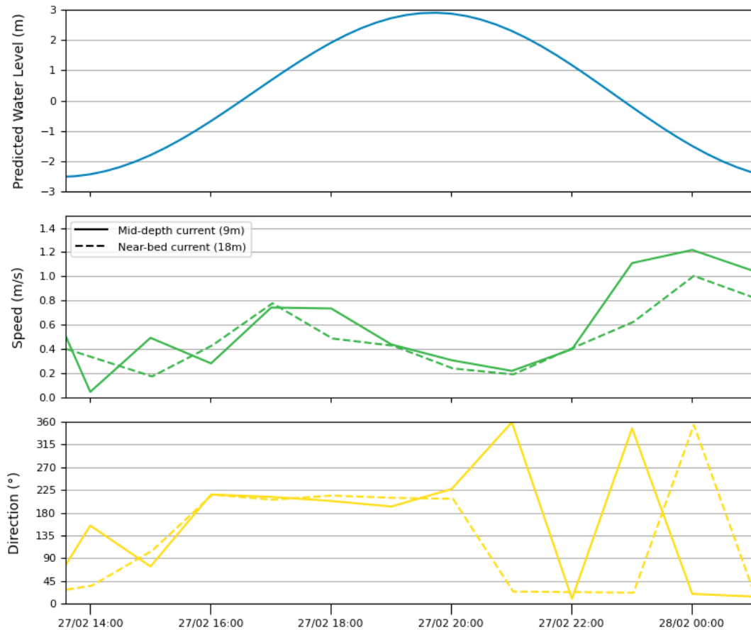
Figure 71. Time series of predicted water level and measured mid depth and near-bed current speed and direction over a spring tide at Site 3.
