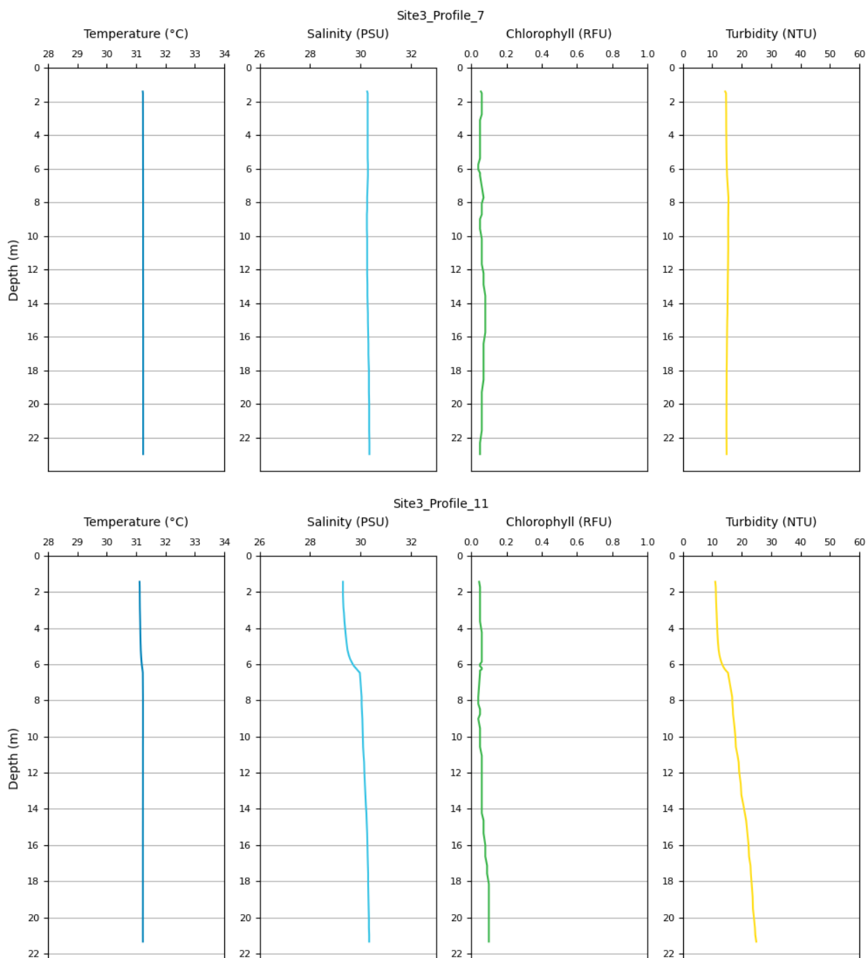
Figure 68. Measured temperature, salinity, chlorophyll and turbidity through the water column at Site 3 at high water (top) and during the ebb stage of the tide (bottom).
