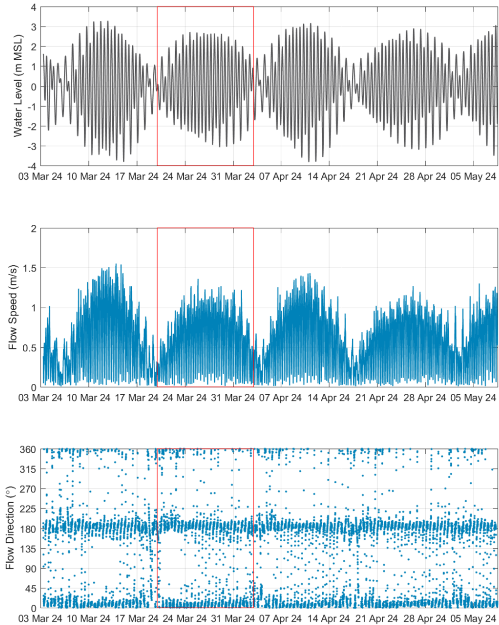
Figure 24. Hydrodynamic survey results for site AWAC-01, 3 rd Mar to 8 th May 2024.
