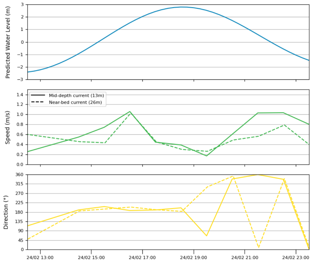
Figure 69. Time series of predicted water level and measured mid depth and near-bed current speed and direction over a spring tide at Site 1.
