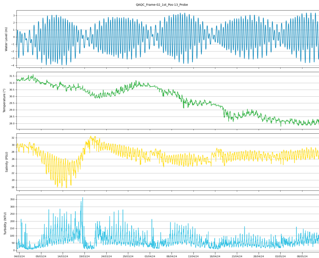
Figure 49. Time series of water level, temperature, salinity and turbidity measured at Pos-13 over the whole deployment period from March to May 2024.
