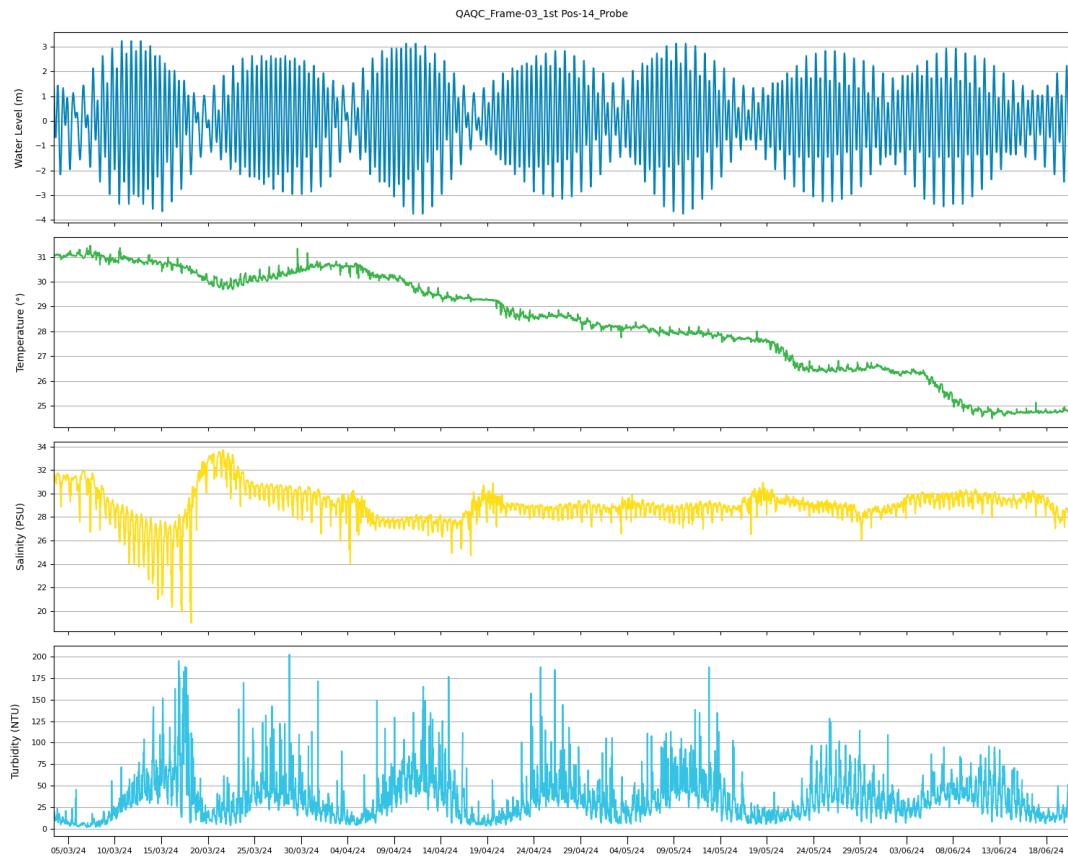
Figure 50. Time series of water level, temperature, salinity and turbidity measured at Pos-14 over the whole deployment period from March to June 2024.
