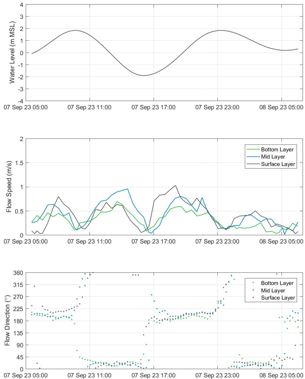
Figure 19. Hydrodynamic survey results for site AWAC-04, 7 th to 8 th Sept 2023.
