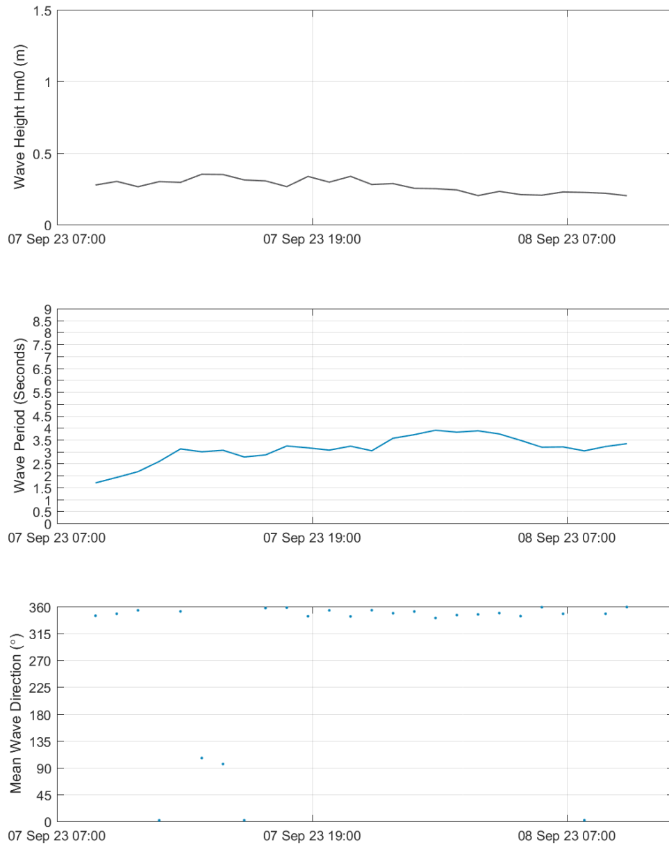
Figure 26. Wave survey results for site AWAC-02, 7 th to 8 th Sept 2023.
