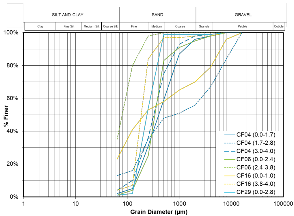
Figure 53. Example plot of PSD from samples within Block 4 of the exploratory campaign.
