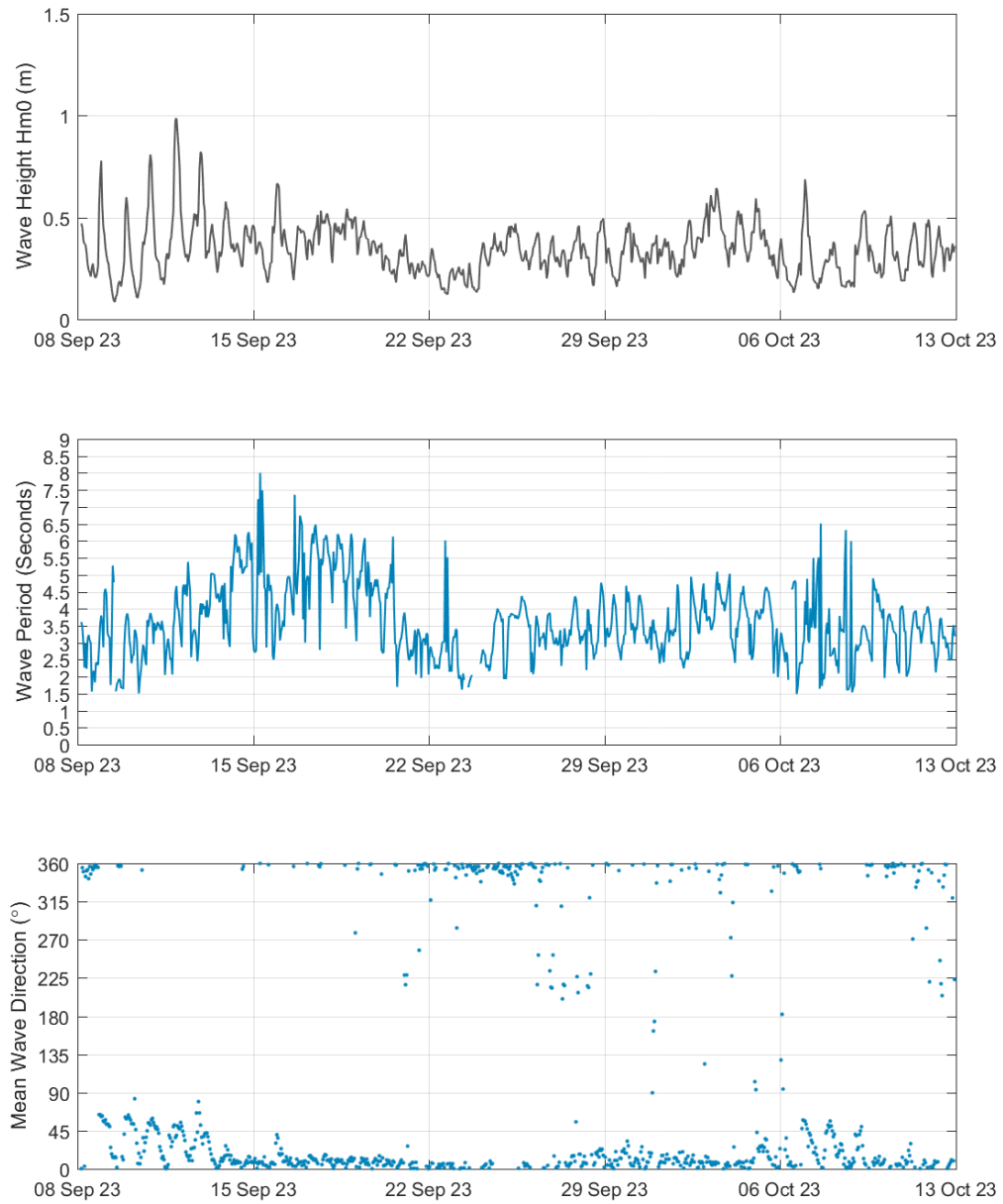
Figure 27. Wave survey results for site AWAC-06, 8 th Sept to 13 th Oct 2023.
