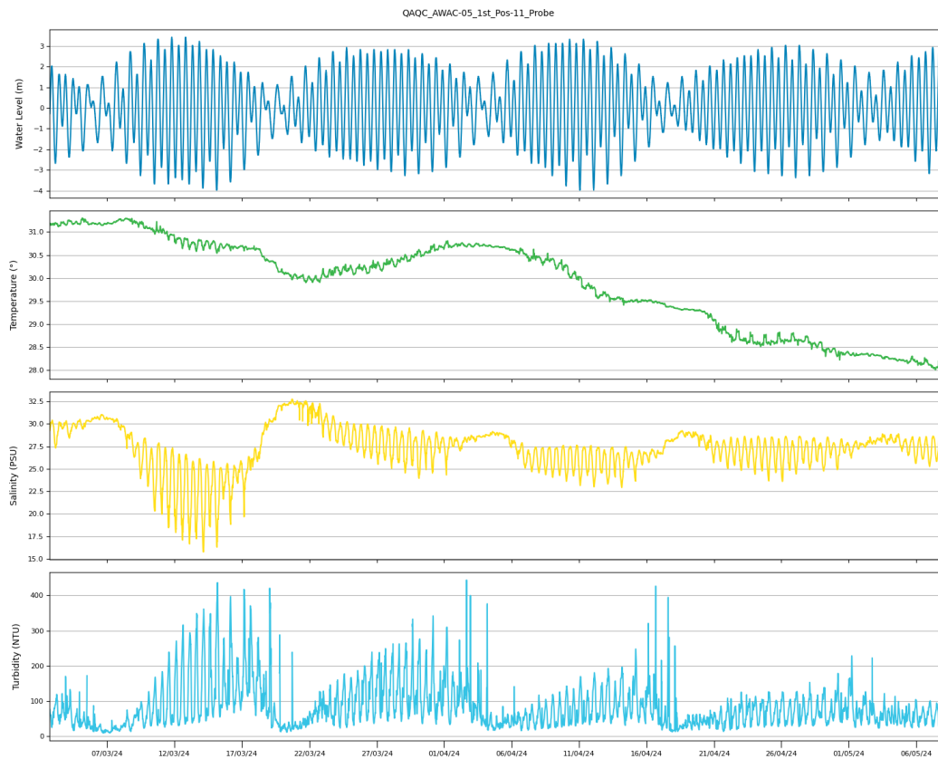
Figure 47. Time series of water level, temperature, salinity and turbidity measured at AWAC-11 over the whole deployment period from March to May 2024.
