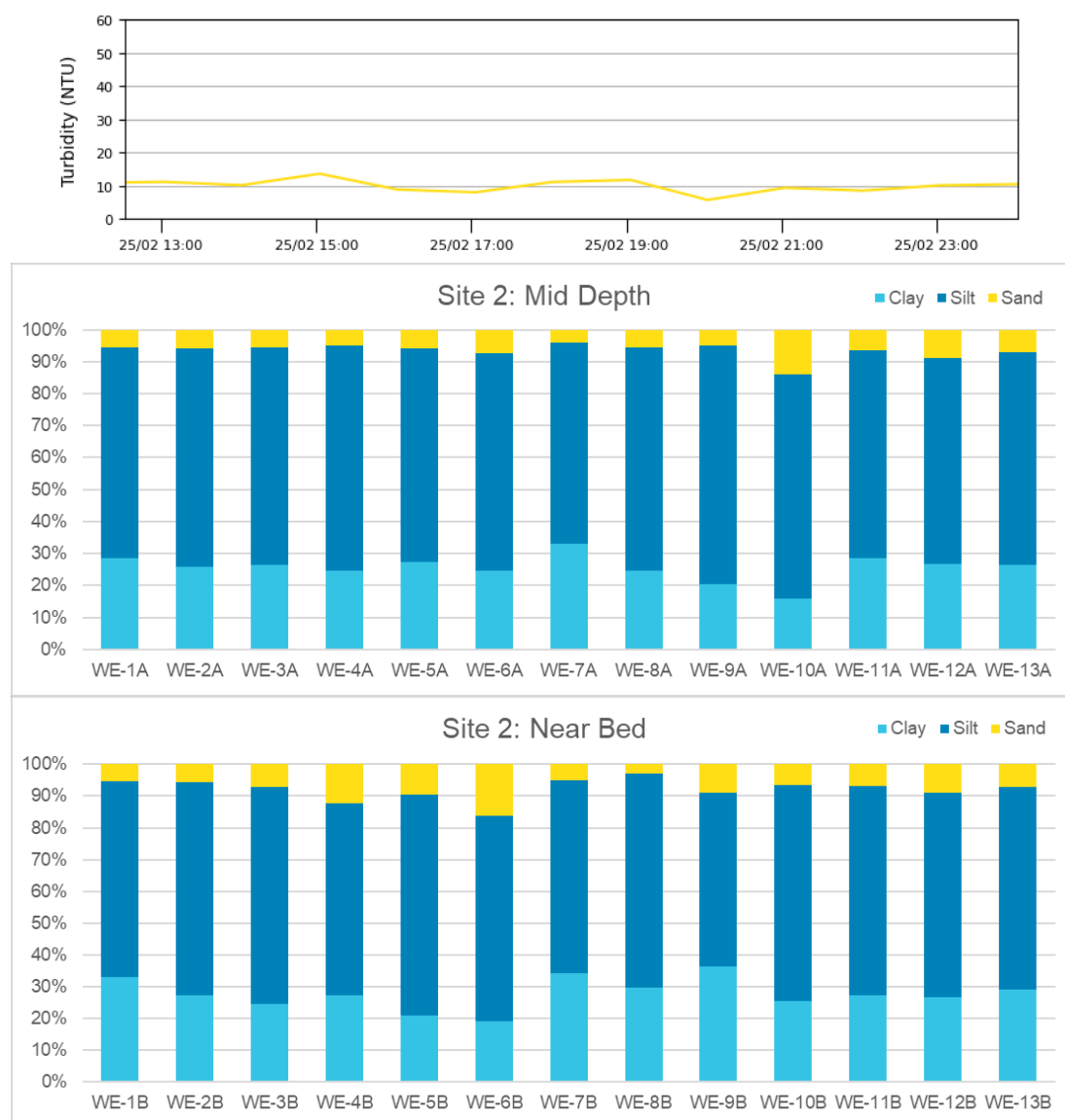
Figure 74. Measured near-bed turbidity (top) and composition of the suspended sediment at mid depth (middle) and near-bed (bottom) over a spring tidal cycle at Site 2. Note: the higher percentage of sand sized particles in samples WE-4B, WE-6B, WE-9B and WE-10A are due to sand sized organic matter being present, the actual percentage of sand will have been in line with the other samples (i.e. 5 to 10%).
