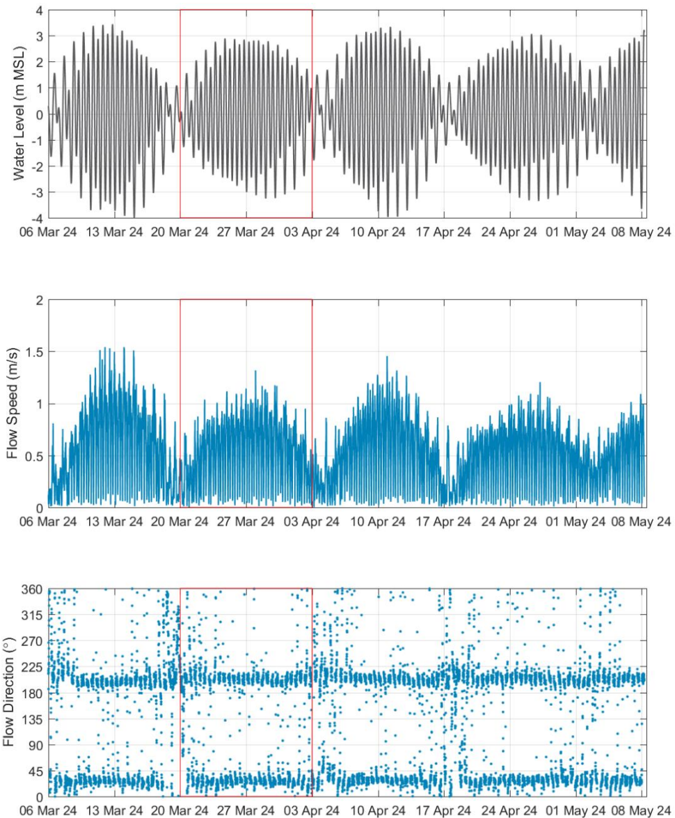
Figure 25. Hydrodynamic survey results for site AWAC-11, 2 nd Mar to 8 th May 2024.
