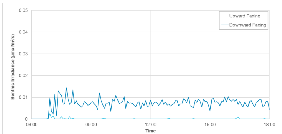
Figure 33. Time series of instantaneous benthic light at AWAC-02 on 07/09/2023.
