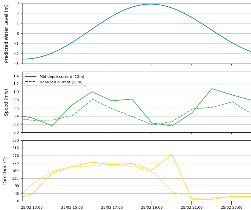
Figure 70. Time series of predicted water level and measured mid depth and near-bed current speed and direction over a spring tide at Site 2.
