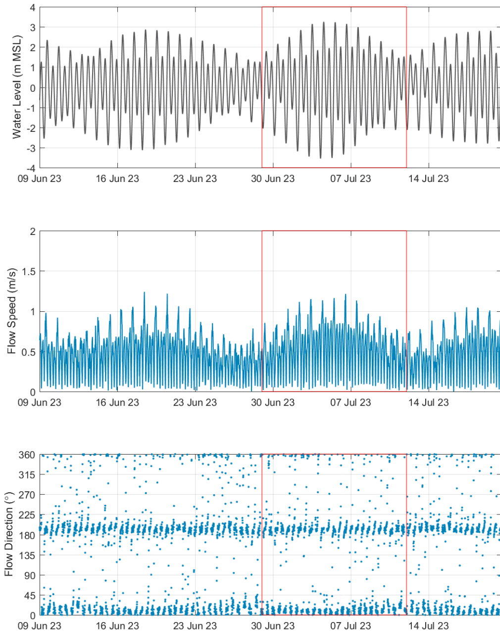
Figure 17. Hydrodynamic survey results for site AWAC-01, 9 th Jun to 21 st Jul 2023.
