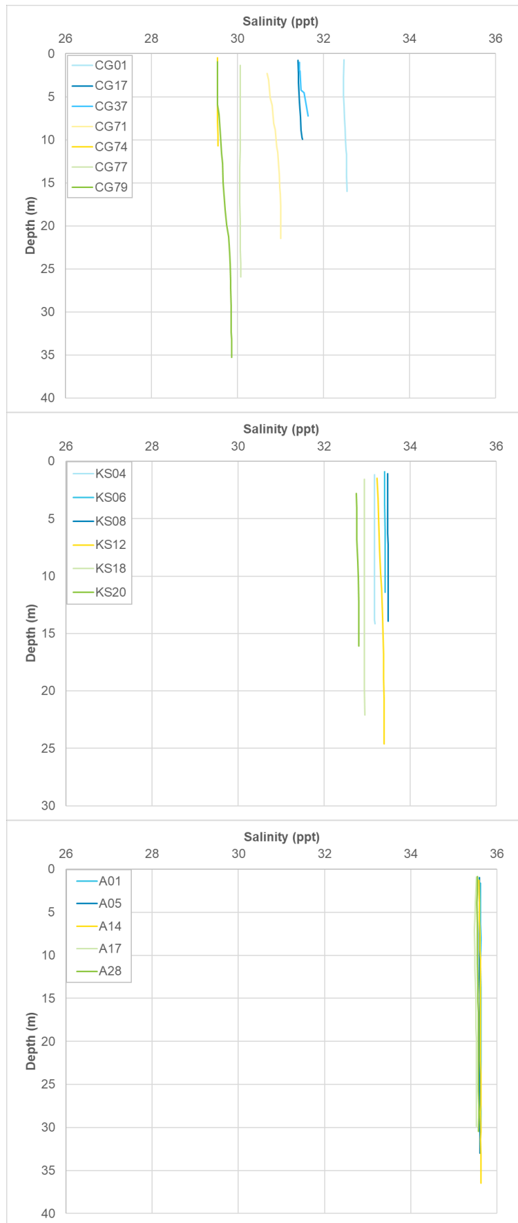
Figure 55. Vertical depth profiles of salinity at sites in CG (top), King Shoals (middle) and offshore (bottom) measured in July-August 2023.
