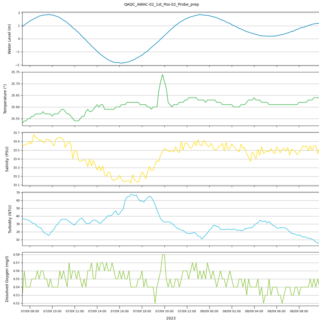
Figure 40. Time series of water level, temperature, salinity and turbidity measured at AWAC-02 in September 2023.
