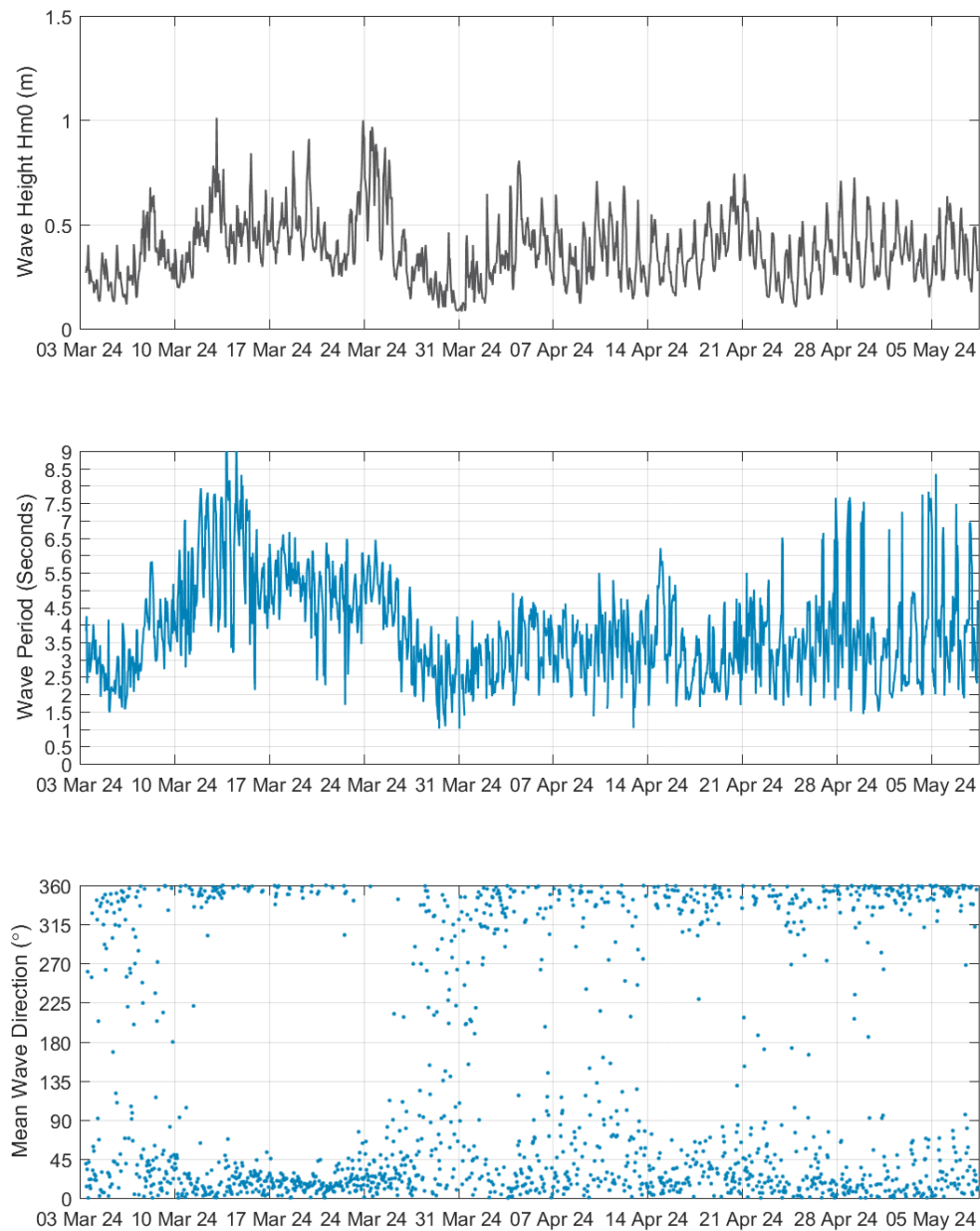
Figure 31. Wave survey results for site AWAC-01, 3 rd Mar to 8 th May 2024.
