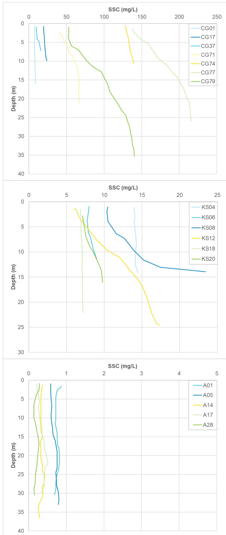
Figure 57. Vertical depth profiles of TSS at sites in the CG (top), King Shoals (middle) and offshore (bottom) measured in July-August 2023.
