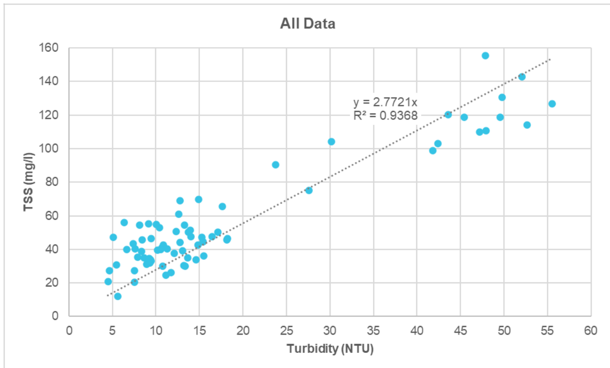
Figure 72. Correlation between measured in-situ turbidity and laboratory calculated TSS for all samples.
