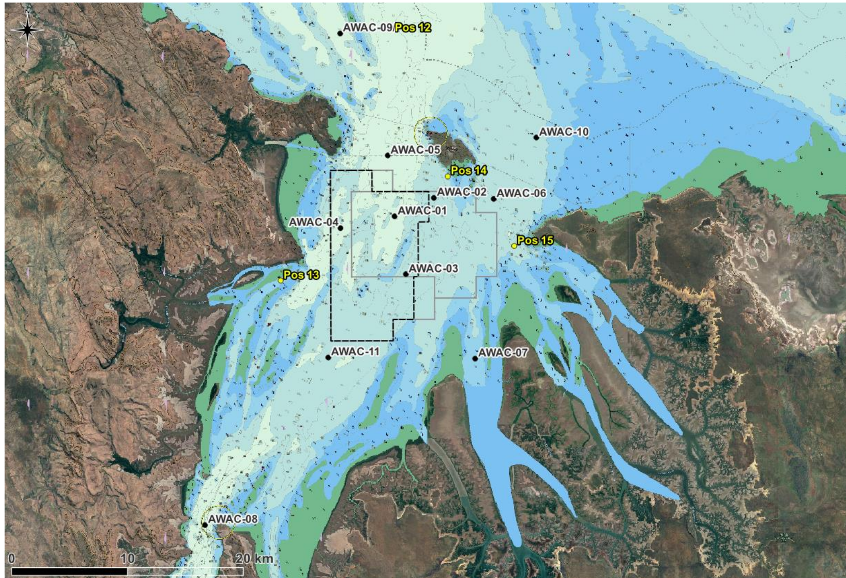
Figure 3. Tens sites where AWACs with co-mounted sensors (AWAC 01 to 11) and fours sited with seabed frames with light & multi-sonde sensors (Pos 12 to 15) have been or are planned to be deployed for the project.
