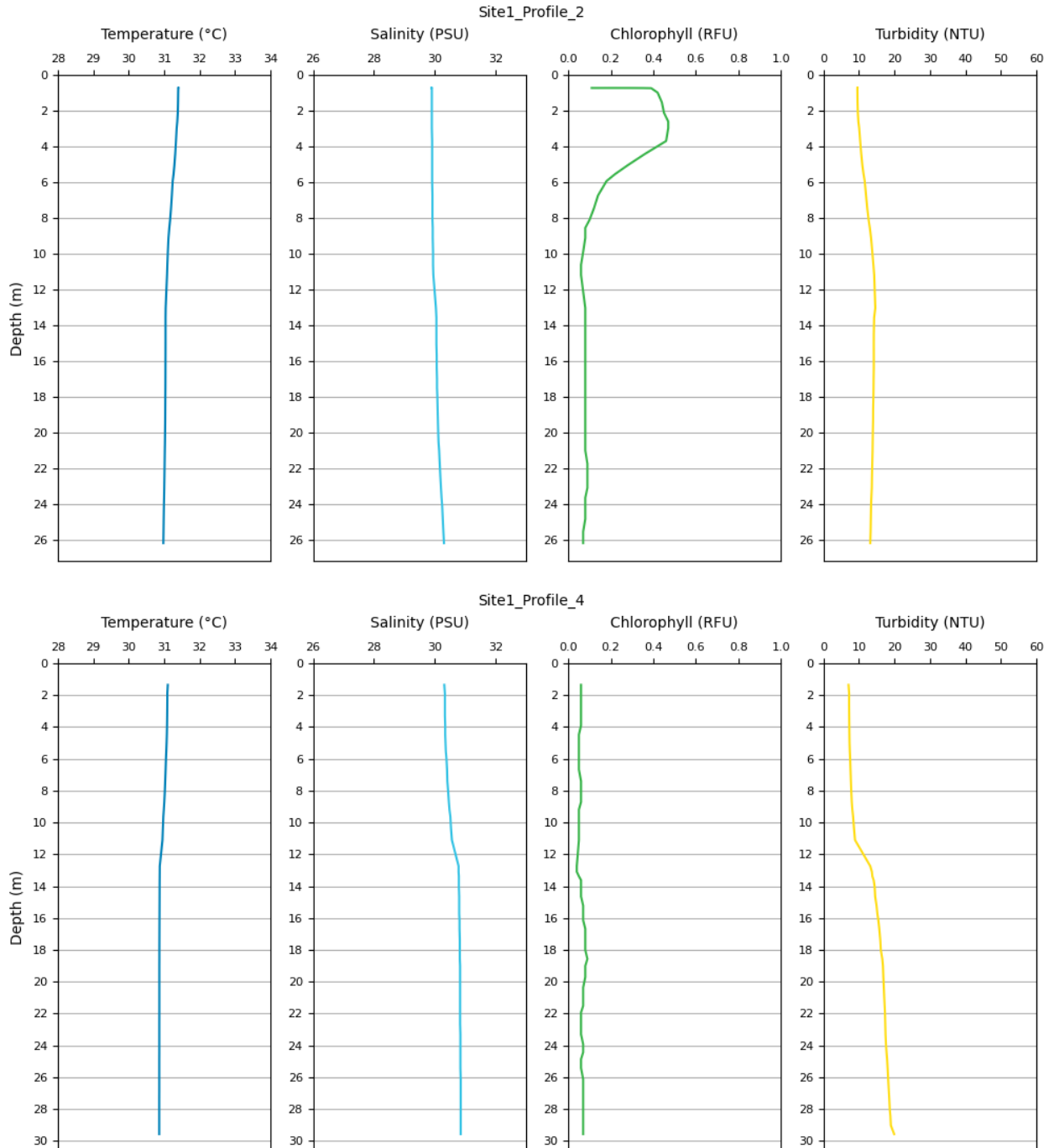
Figure 63. Measured temperature, salinity, chlorophyll and turbidity through the water column at Site 1 close to low water (top) and during the flood stage of the tide (bottom).
