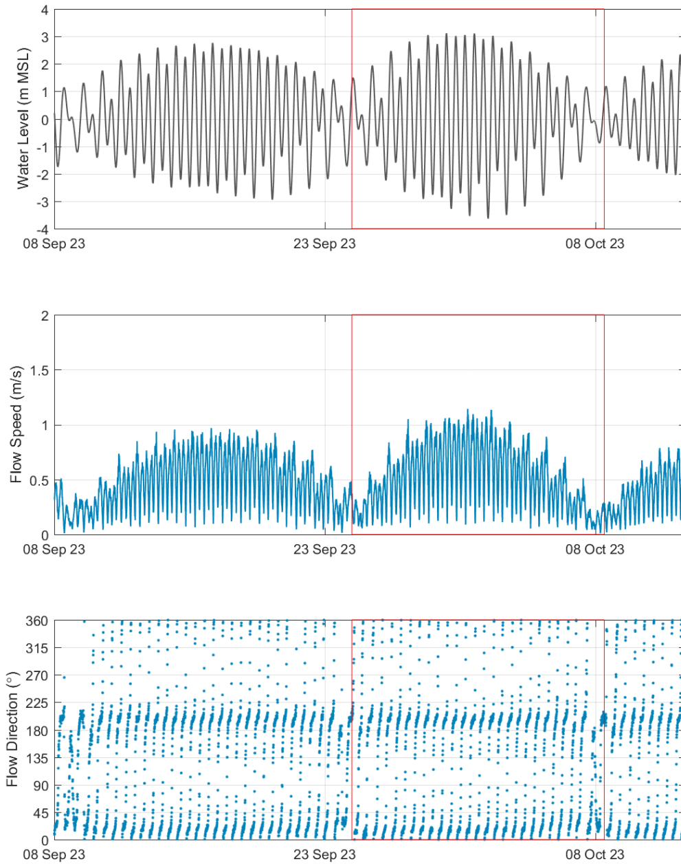
Figure 20. Hydrodynamic survey results for site AWAC-06, 8 th Sept to 13 th Oct 2023.
