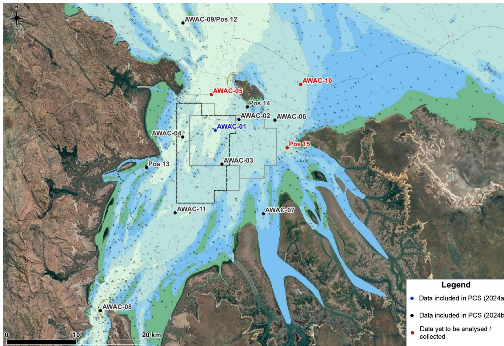
Figure 14. Sites where AWACs with co-mounted sensors (AWAC 01 to 11) and seabed frames with light & turbidity sensors (Pos 12 to 15) have been or are planned to be deployed for the project.
