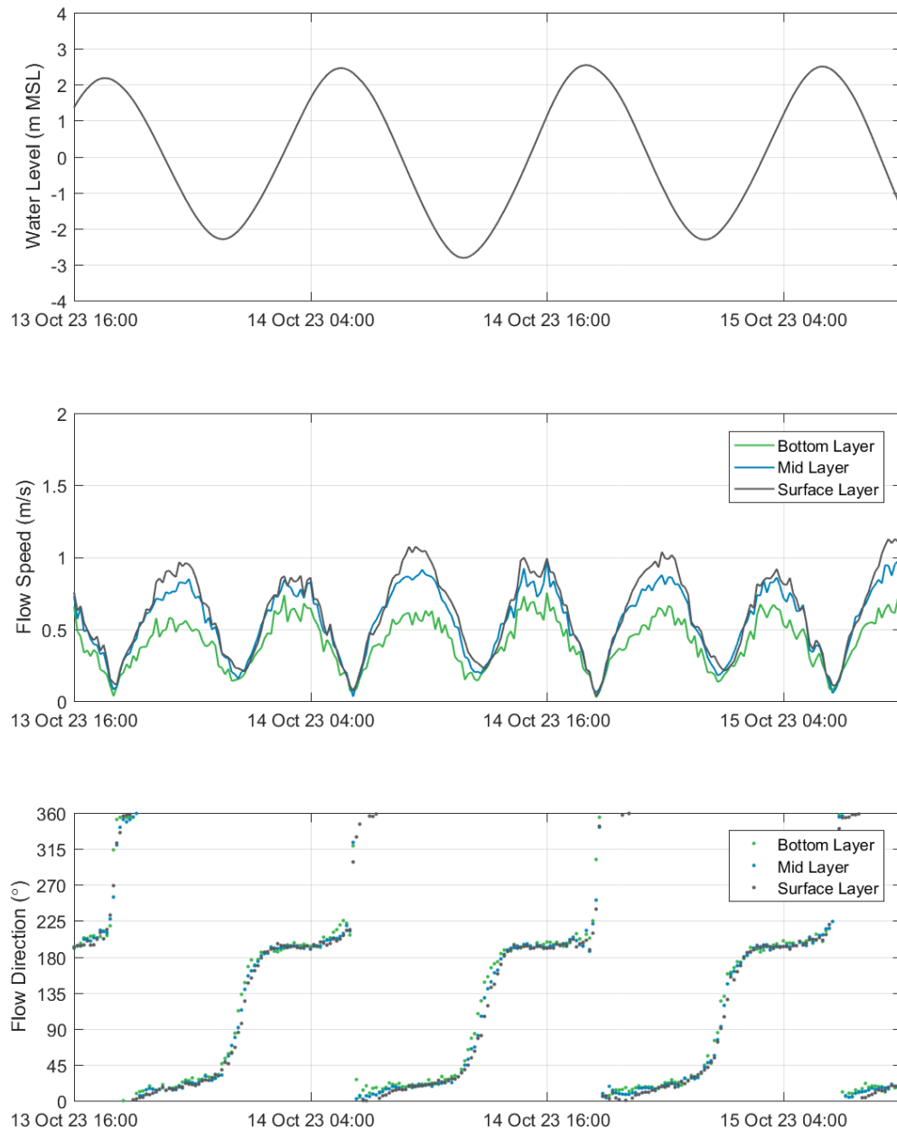
Figure 21. Hydrodynamic survey results for site AWAC-03, 13 th to 15 th Oct 2023.
