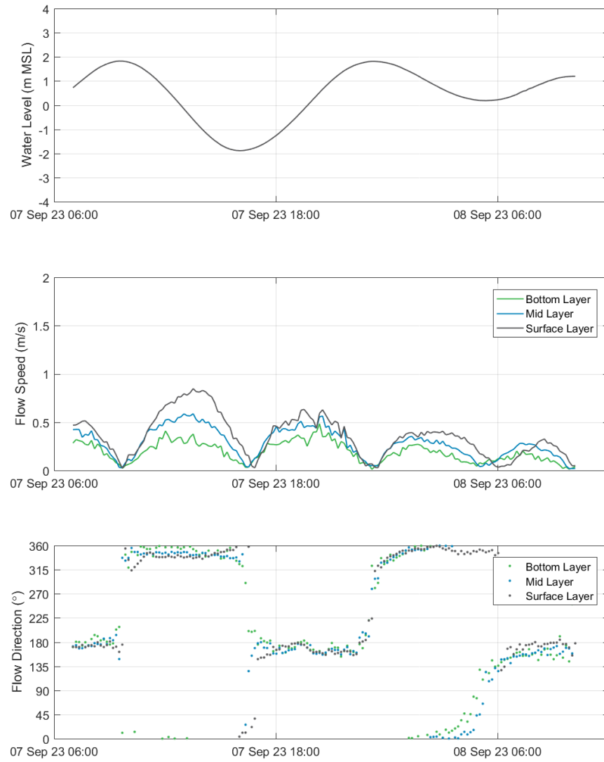
Figure 18. Hydrodynamic survey results for site AWAC-02, 7 th to 8 th Sept 2023.
