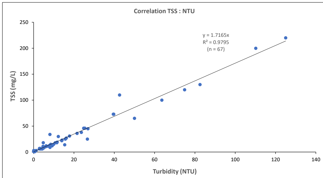
Figure 58. Site-specific relationship between measured Turbidity (NTU) values and analysed Total Suspended Solids (TSS) concentrations (in mg/L) for Cambridge Gulf (dry season).
