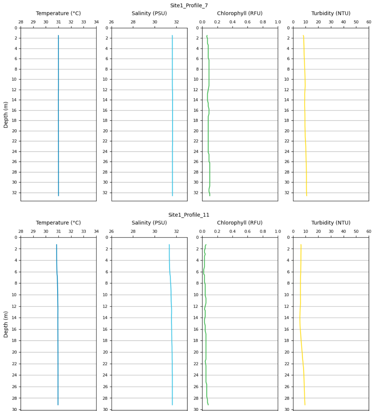
Figure 64. Measured temperature, salinity, chlorophyll and turbidity through the water column at Site 1 at high water (top) and during the ebb stage of the tide (bottom).
