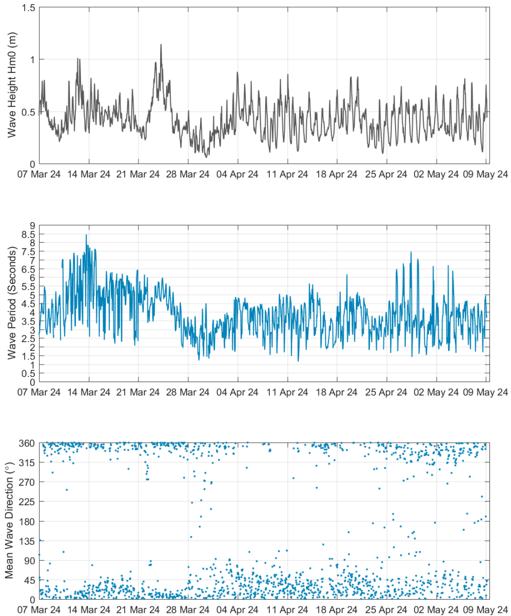
Figure 30. Wave survey results for site AWAC-06 (Second deployment), 6 th Mar to 10 th May 2024.
