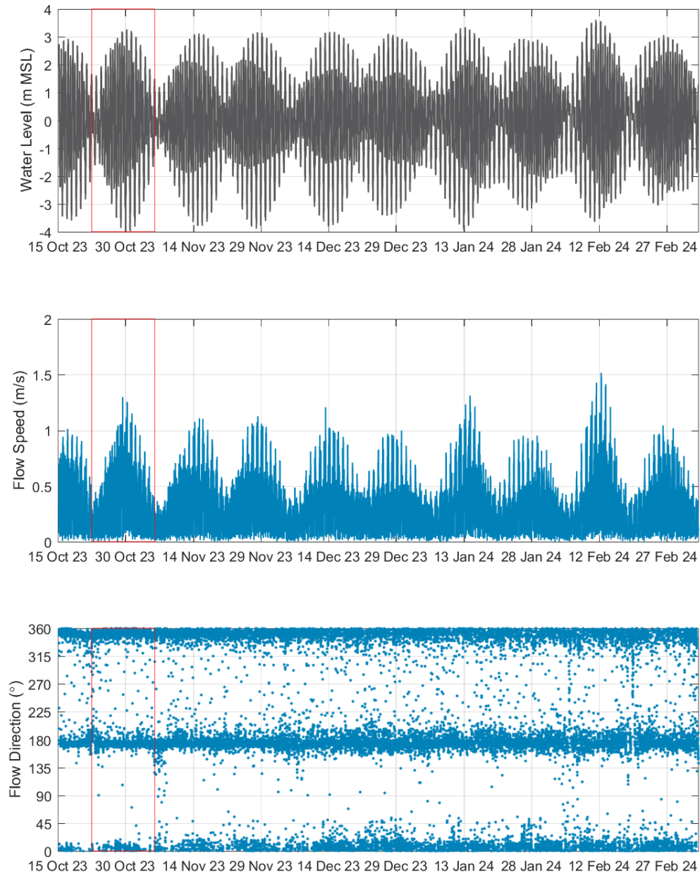
Figure 22. Hydrodynamic survey results for site AWAC-07, 15 th Oct 2023 to 5 th Mar 2024.
