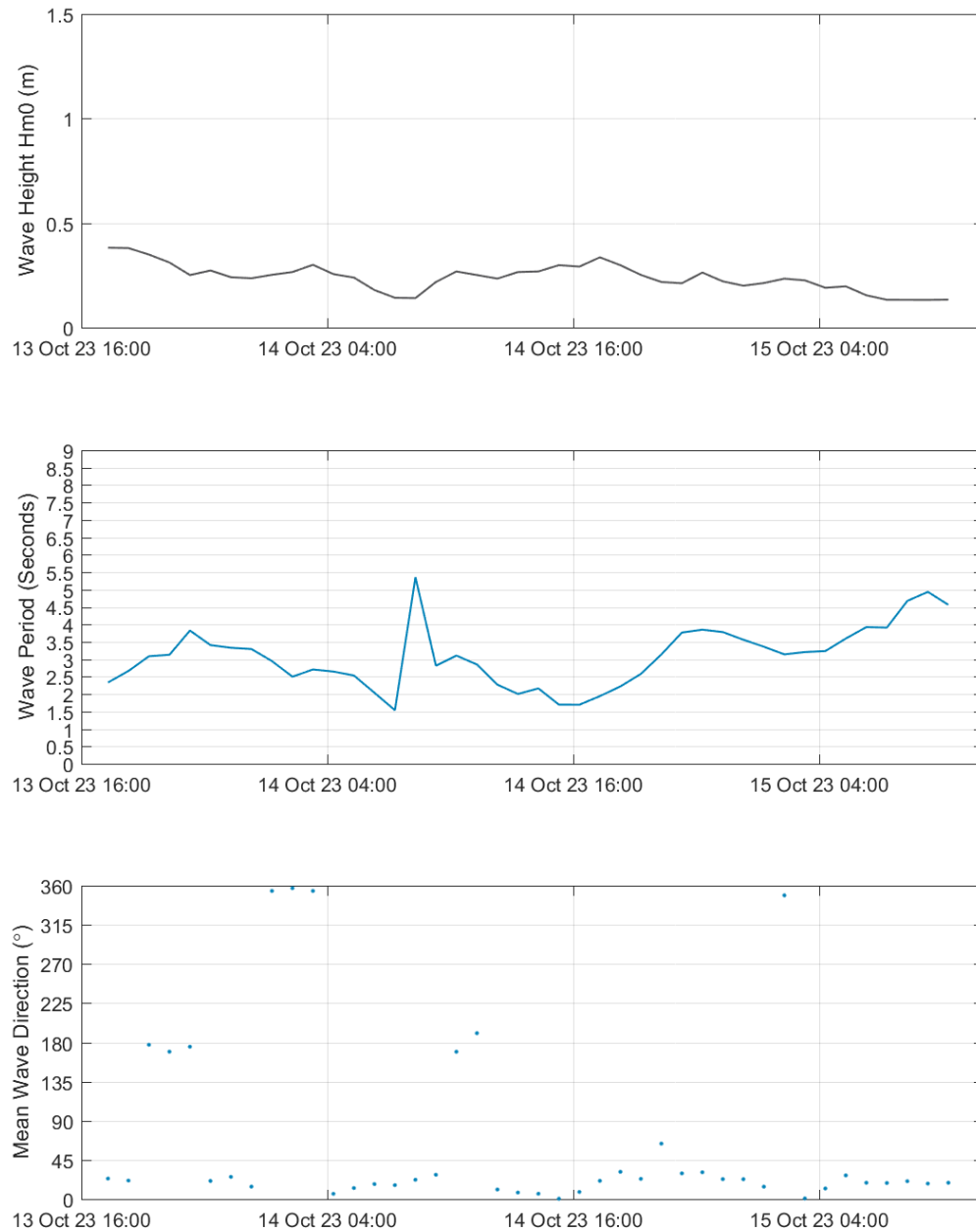
Figure 28. Wave survey results for site AWAC-03, 13 th to 15 th Oct 2023.
