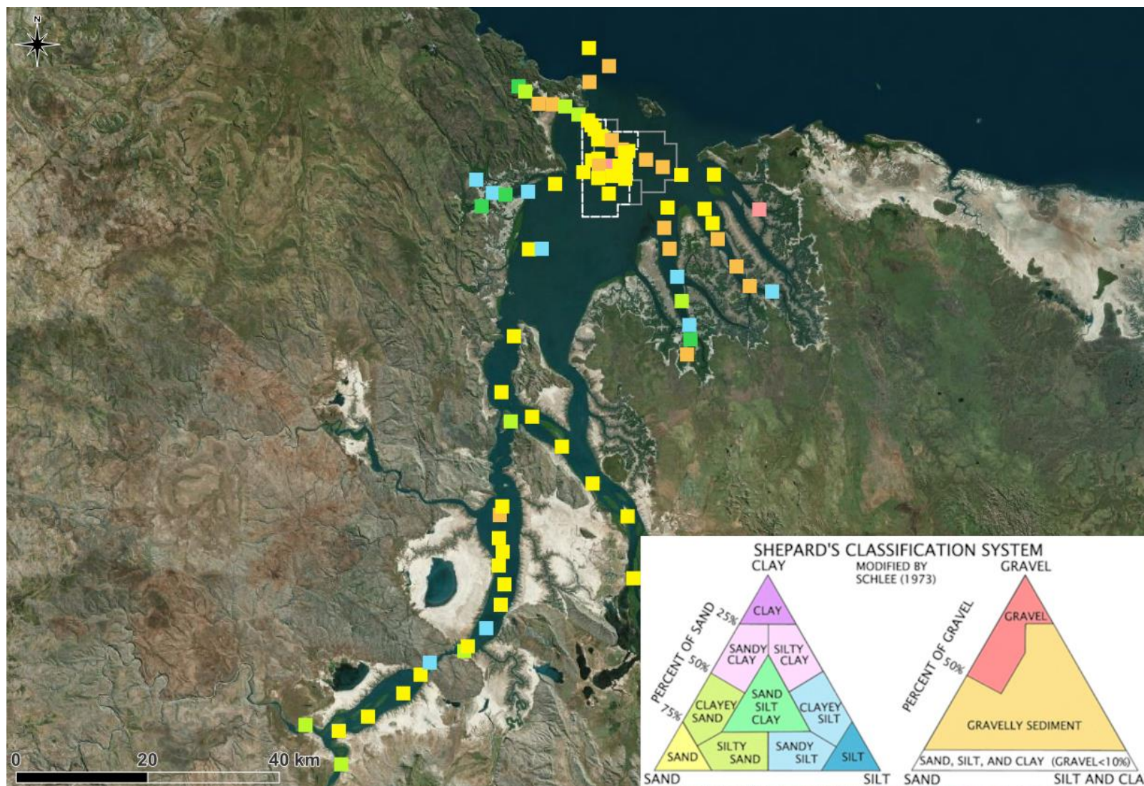
Figure 60. Map showing sediment type for all samples based on Shepard's classification system using the percentage of clay, silt, sand and gravel in the sample.
