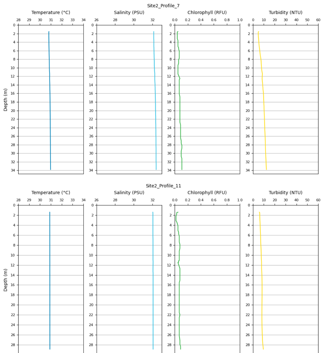
Figure 66. Measured temperature, salinity, chlorophyll and turbidity through the water column at Site 2 at high water (top) and during the ebb stage of the tide (bottom).
