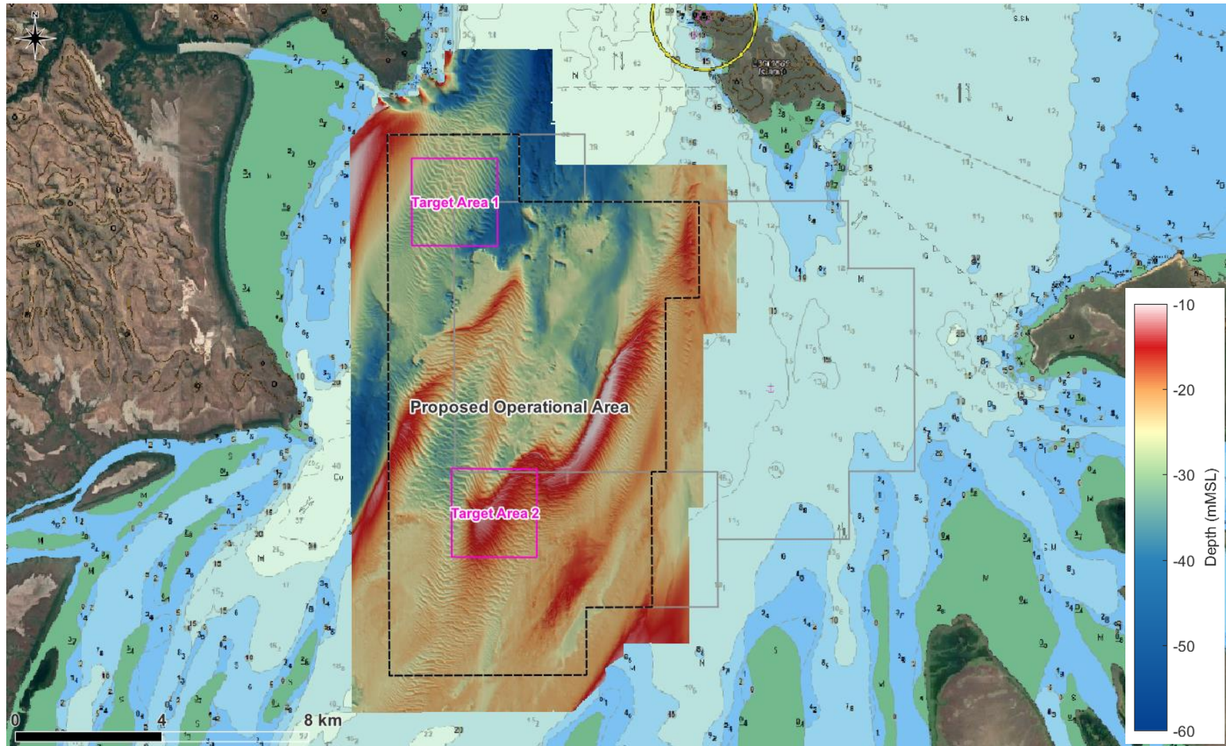
Figure 9. Multibeam bathymetric survey extent along with Areas 1 and 2. Note: the black dashed line shows the proposed operational area.
