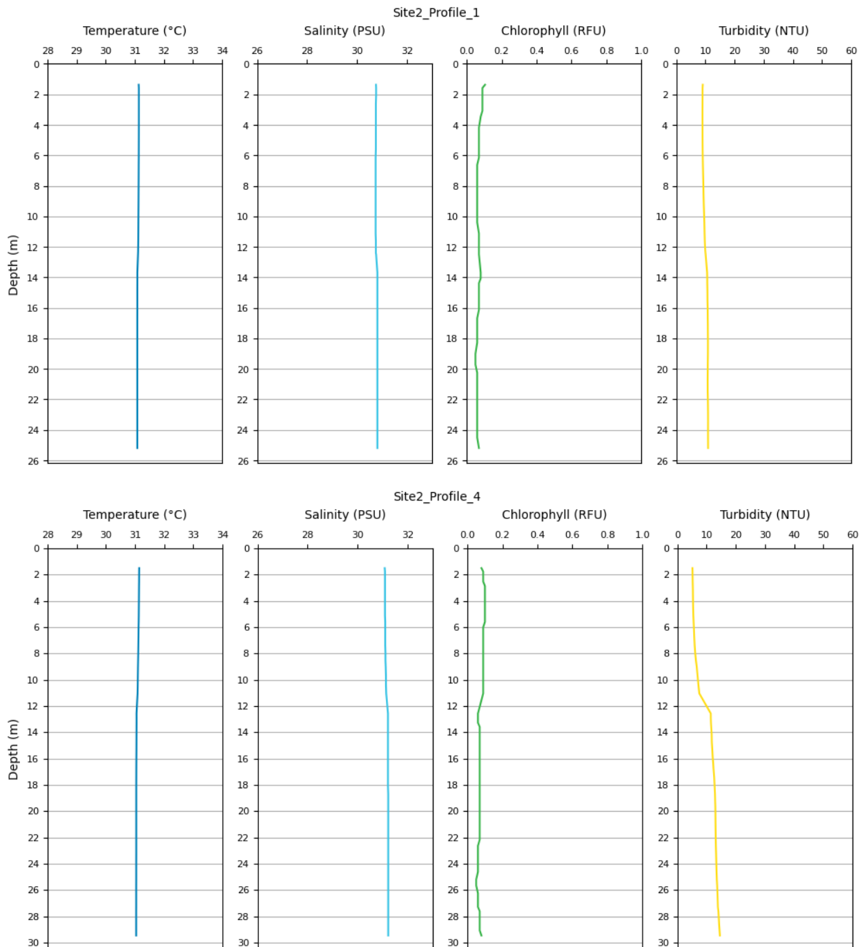
Figure 65. Measured temperature, salinity, chlorophyll and turbidity through the water column at Site 2 at low water (top) and during the flood stage of the tide (bottom).
