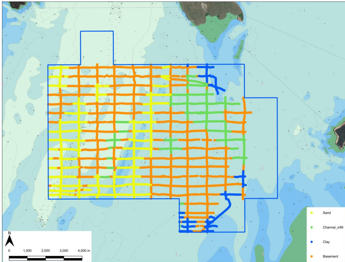
Figure 51. Sediment types within Block 4 based on the sub-bottom profiling and sidescan sonar data.
