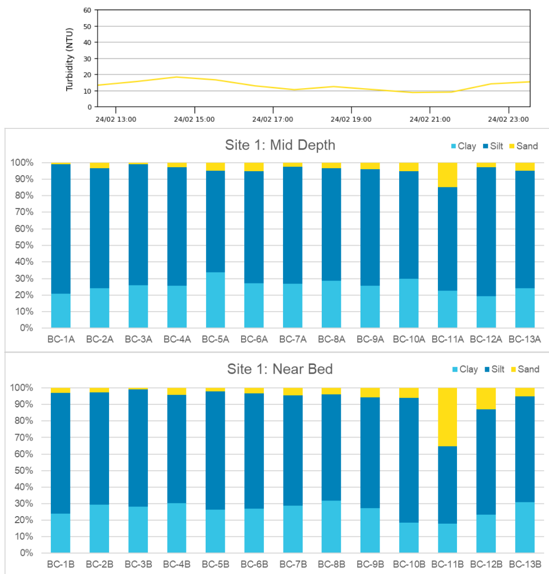
Figure 73. Measured near-bed turbidity (top) and composition of the suspended sediment at mid depth (middle) and near-bed (bottom) over a spring tidal cycle at Site 1. Note: the high percentage of sand sized particles in samples BC-11A, BC-11B and BC-12B are due to sand sized organic matter being present, the actual percentage of sand will have been in line with the other samples (i.e. around 5%).
