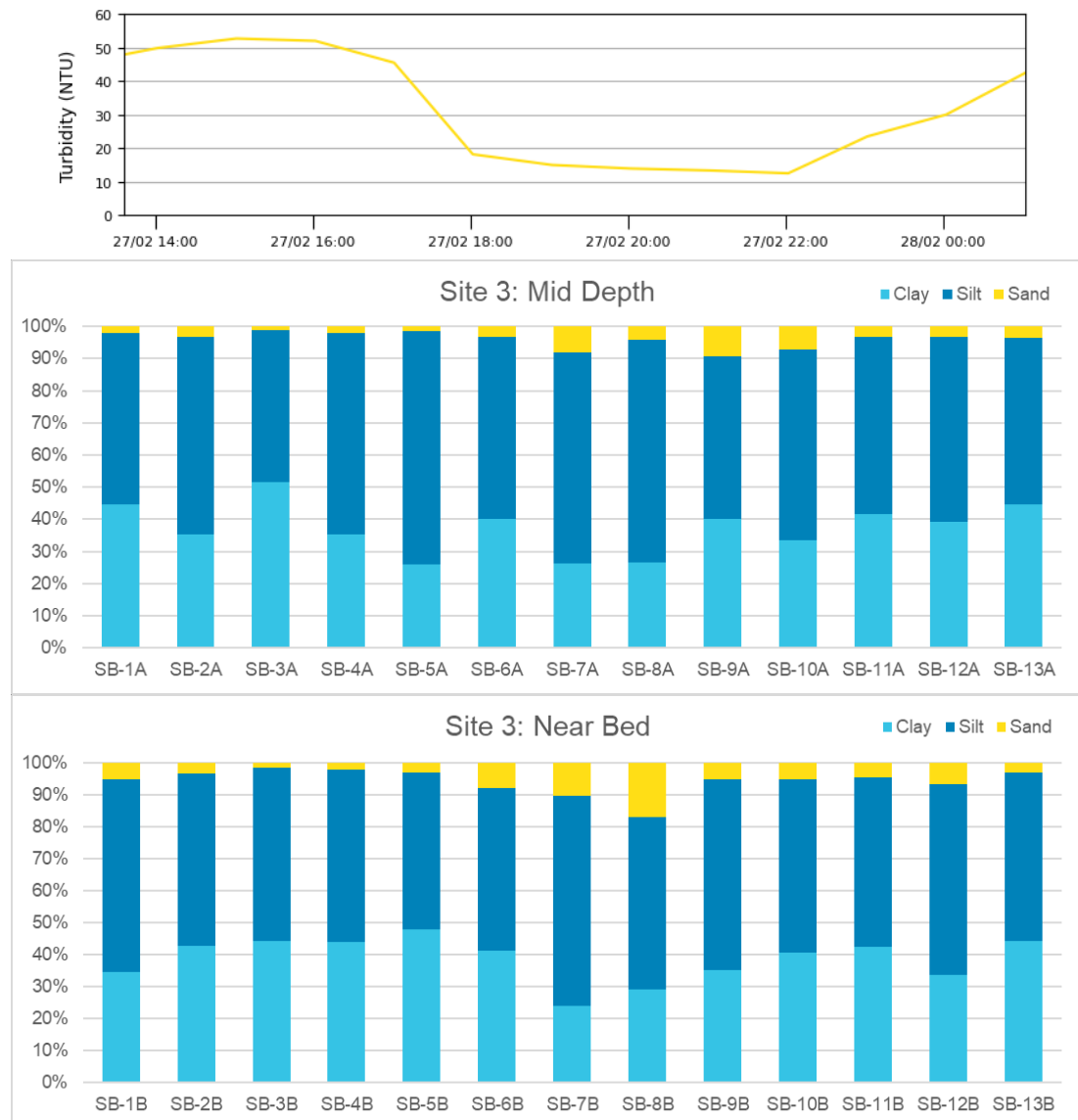
Figure 75. Measured near-bed turbidity (top) and composition of the suspended sediment at mid depth (middle) and near-bed (bottom) over a spring tidal cycle at Site 3. Note: the higher percentage of sand sized particles in samples SB-7A, SB-7B, SB-8B and SB-9A are due to sand sized organic matter being present, the actual percentage of sand will have been in line with the other samples (i.e. around 5%).
