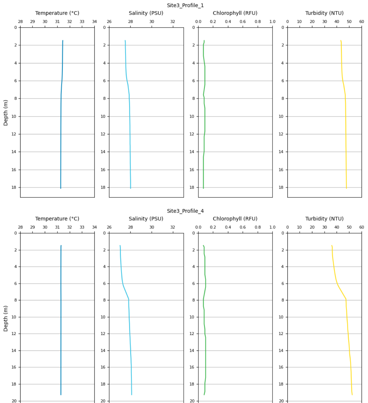
Figure 67. Measured temperature, salinity, chlorophyll and turbidity through the water column at Site 3 at low water (top) and during the flood stage of the tide (bottom).
