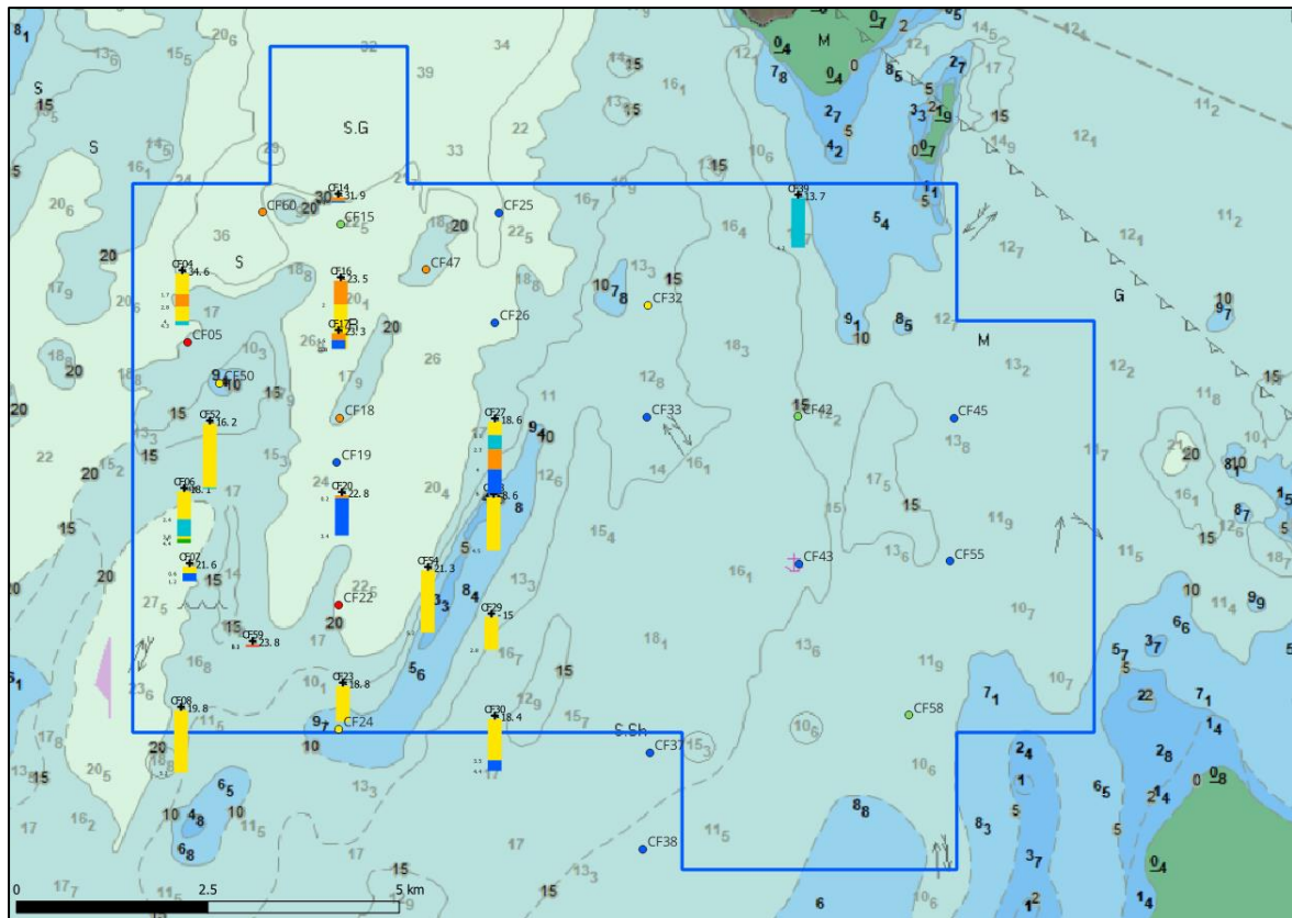
Figure 52. Sediment core data within Block 4 based on the vibro-coring results.
