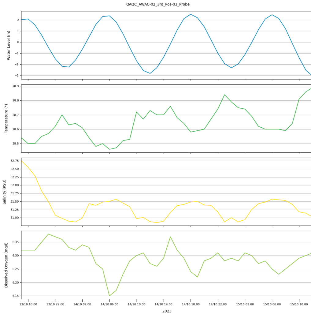
Figure 42. Time series of water level, temperature, salinity and dissolved oxygen measured at AWAC-03 in October 2023.
