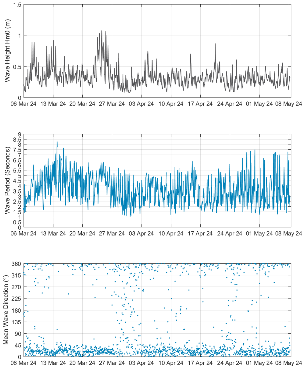
Figure 32. Wave survey results for site AWAC-11, 2 nd Mar to 8 th May 2024.
