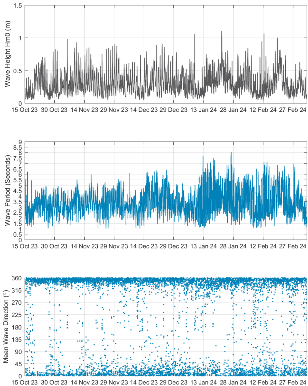
Figure 29. Wave survey results for site AWAC-07, 15 th Oct 2023 to 5 th Mar 2024.
