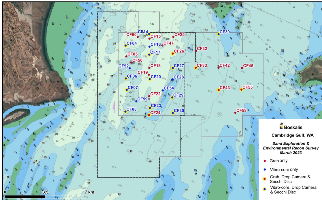
FIGURE 16: The locations of the 16 vibrocore samples taken in March 2023 (refer legend).
